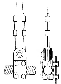
⑬ Cable network; edge cable clamp
